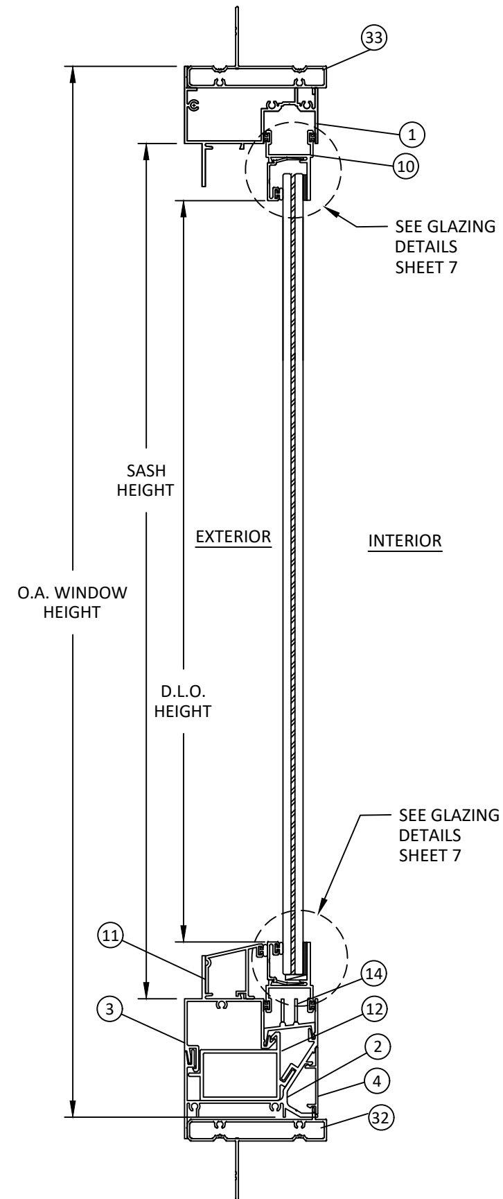
C 4 VERTICAL SECTION LAMINATED GLASS OPERABLE PANEL WITH FIN CLIP ADAPTER LAMINATED GLASS SHOWN. INSULATED LAMINATED GLASS QUALIFIED
