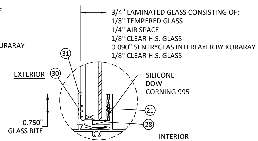
GLAZING DETAIL 2 (G2) SERIES 2062
