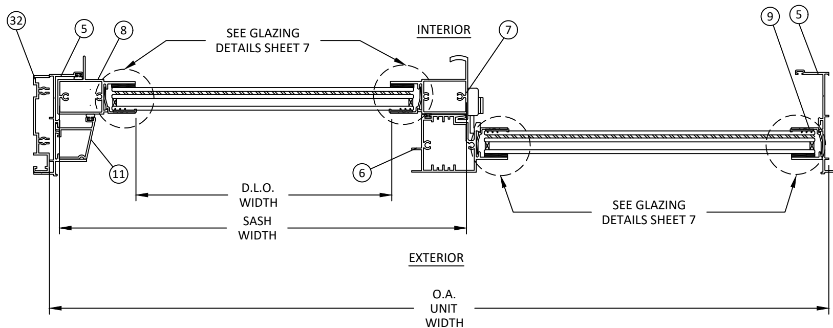
B HORIZONTAL SECTION 5 INSULATED LAMINATED GLASS WITH OPTIONAL LEG ADAPTER
