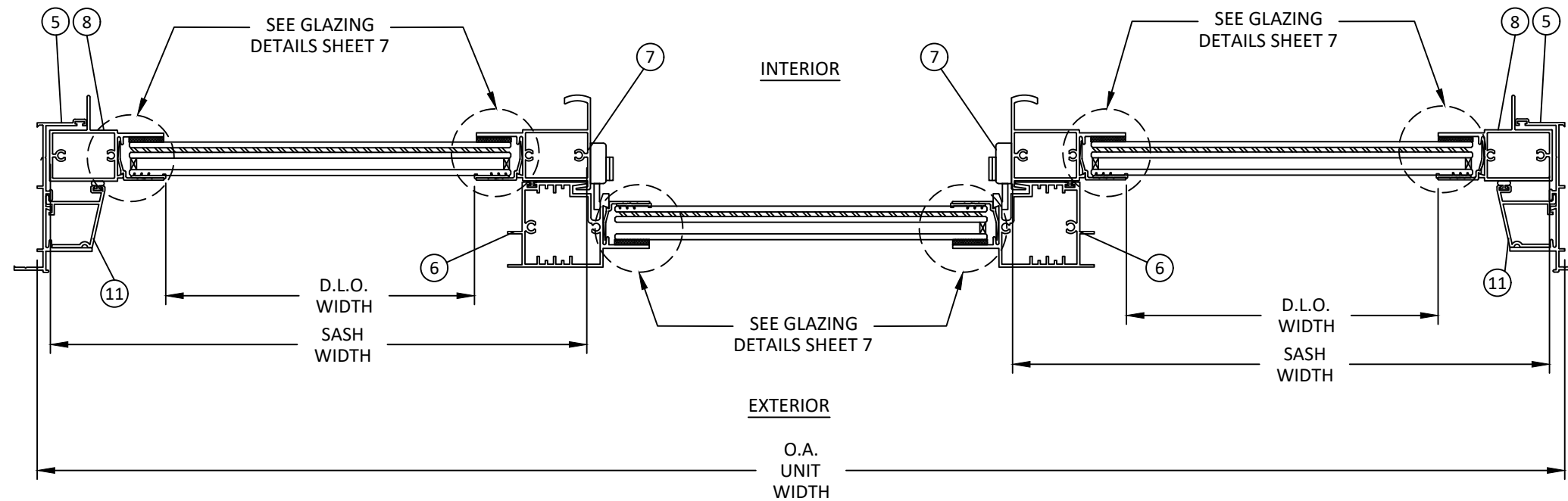
B HORIZONTAL SECTION 6 INSULATED LAMINATED GLASS
