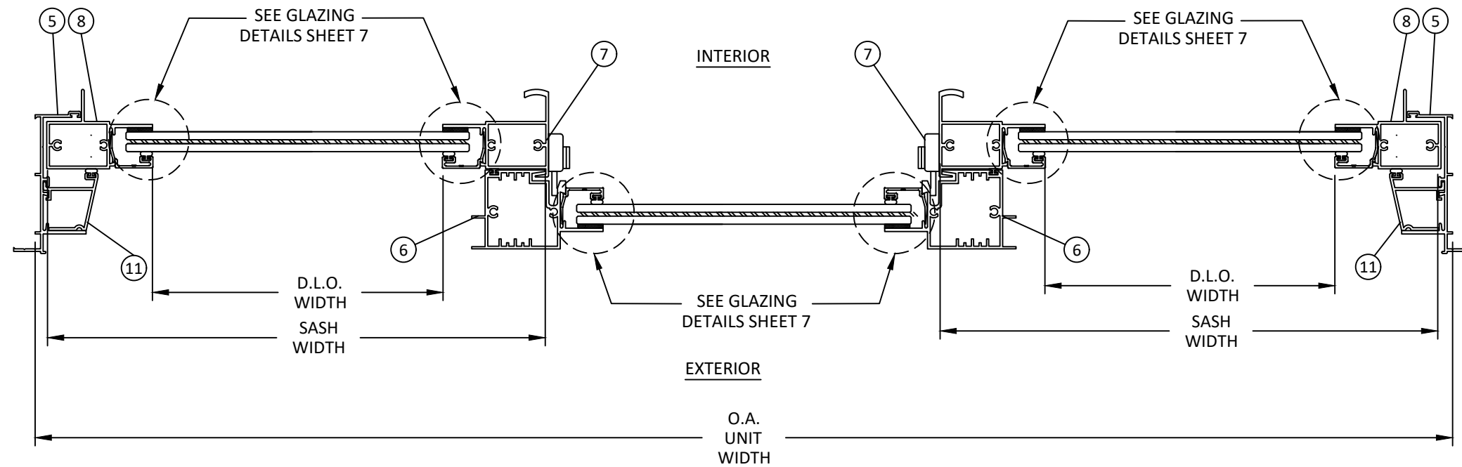
A HORIZONTAL SECTION 6 LAMINATED GLASS
