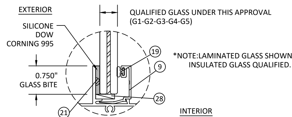
FIXED UNIT GLAZING
