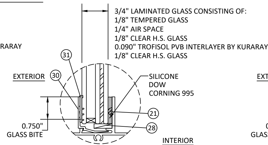
GLAZING DETAIL 1 (G1) SERIES 2041
