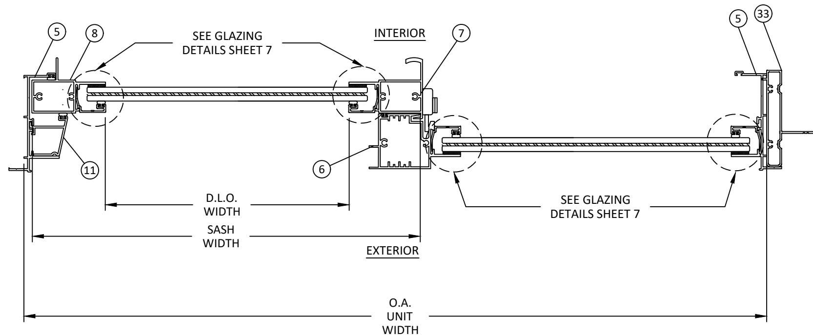
A HORIZONTAL SECTION 5 LAMINATED GLASS WITH OPTIONAL FIN CLIP ADAPTER
